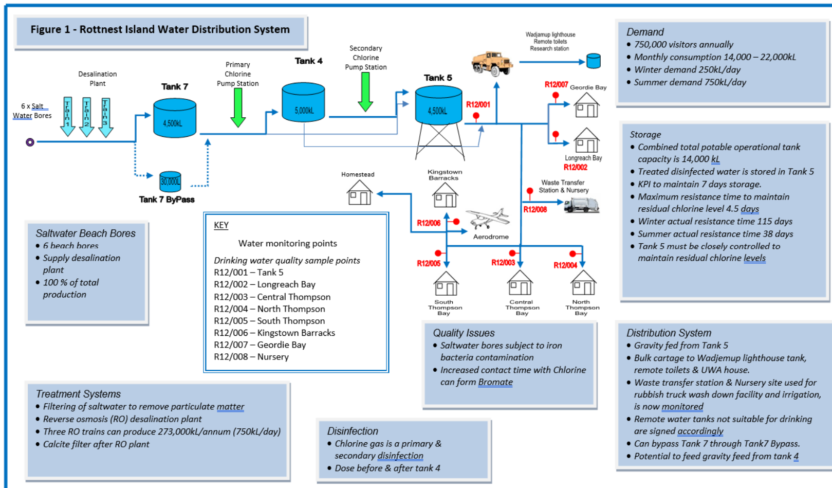
Figure 1: Rottnest Island Water Distribution System
