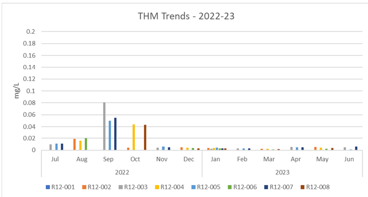
Figure B.2: THM trends during the 2022 – 23 monitoring period (ADWG limit 0.25 mg/L)
