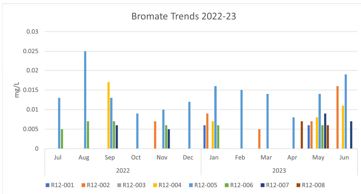
Figure B.1: Bromate trends during the 2022 – 23 monitoring period (ADWG limit 0.02 mg/L).
