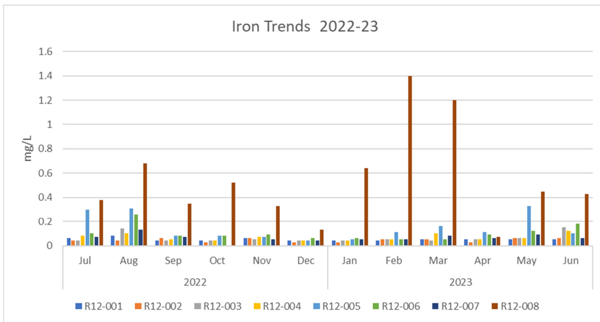
Figure C.2: Iron trends during the 2022 – 23 monitoring period (ADWG limit 0.3 mg/L)
