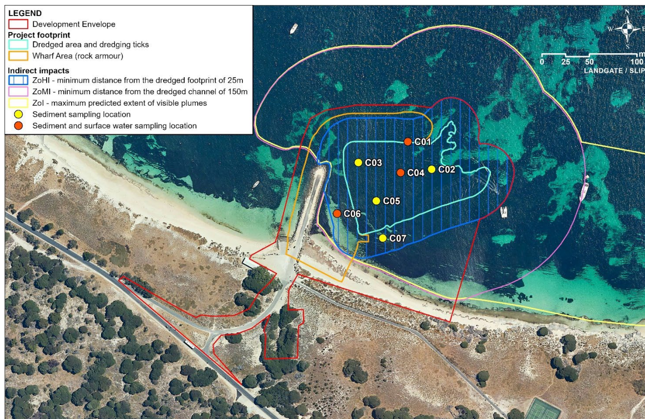
Figure 25: Baseline marine sediment sampling locations
