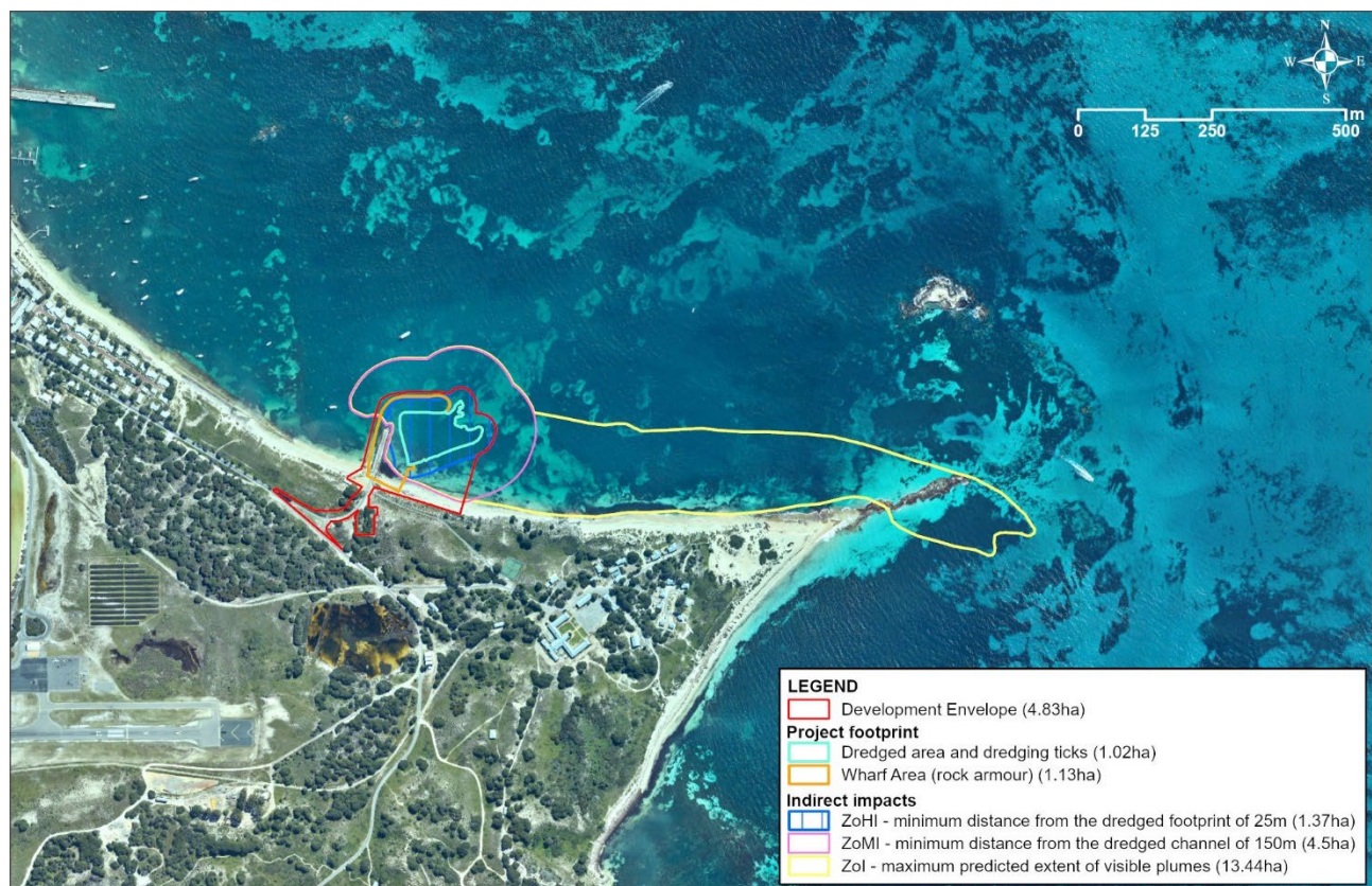
Figure 26: Zones of influence from dredging activities
