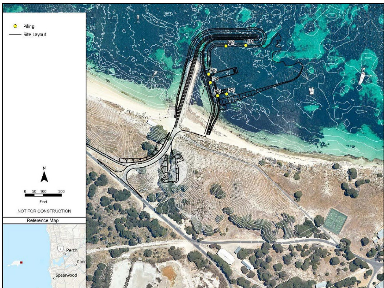
Figure 30: Underwater noise modelling – piling locations
