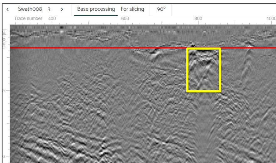
Figure 11: Processed radar-gram (2D cross-section) of the identified soak well feature at depth. The red line sits at a depth of 0.7m.
